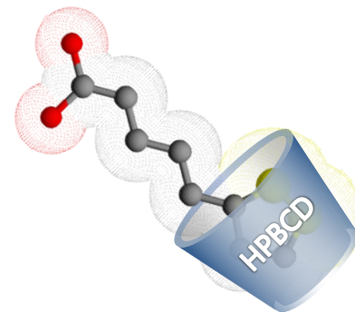
Lipoic acid in HPBCD
